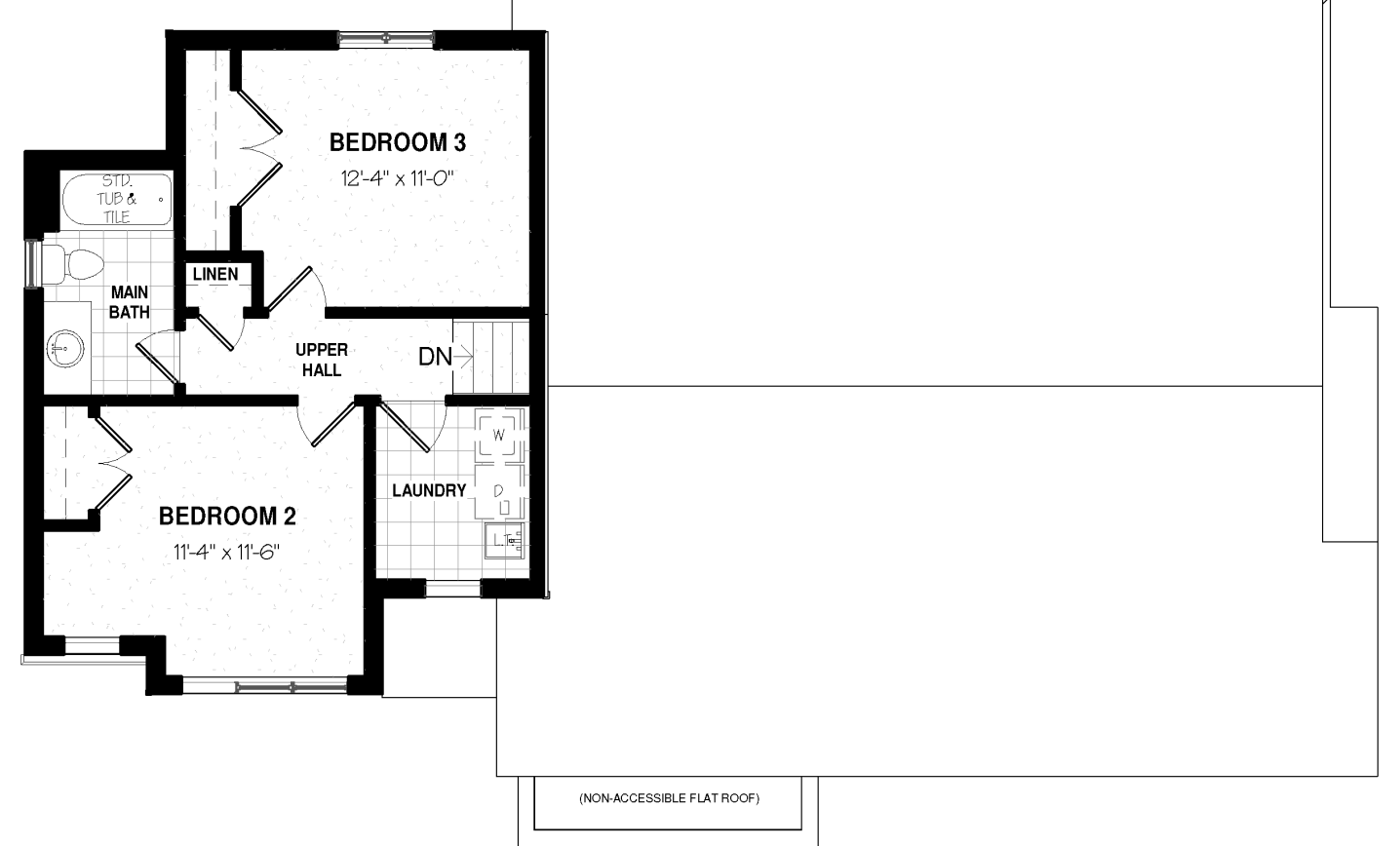
SECOND FLOOR PLAN - 552 sq. ft.
