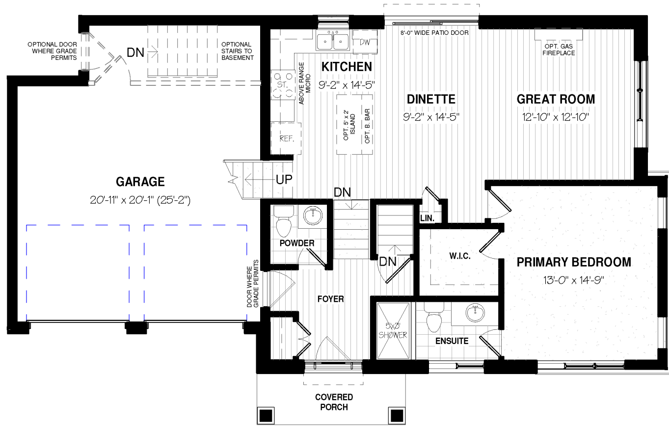
MAIN FLOOR PLAN - 995 sq. ft.
