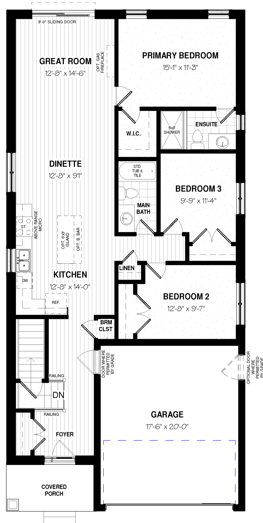
MAIN FLOOR PLAN -1413 sq. ft.
