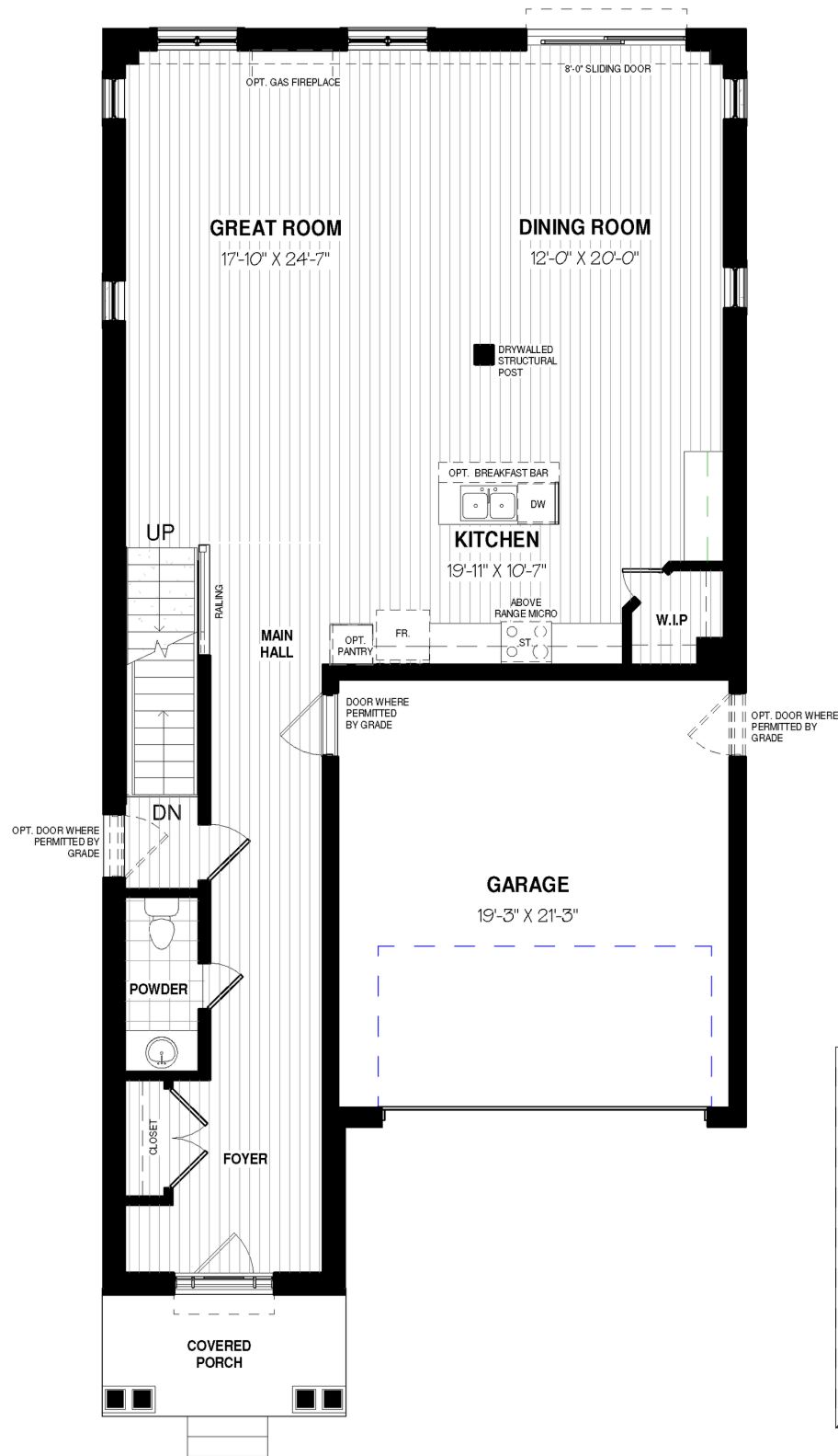
MAIN FLOOR PLAN-1396 sq.ft.
