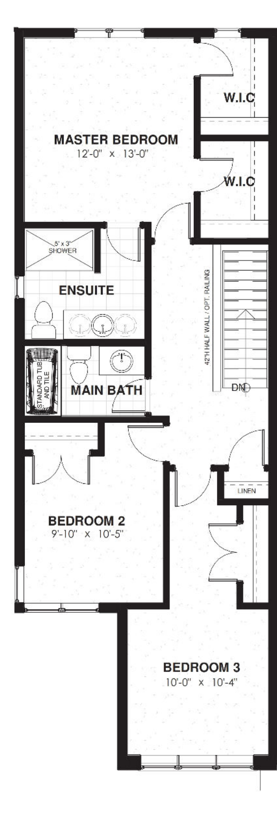
2ND FLOOR PLAN - 841 sq. ft.
