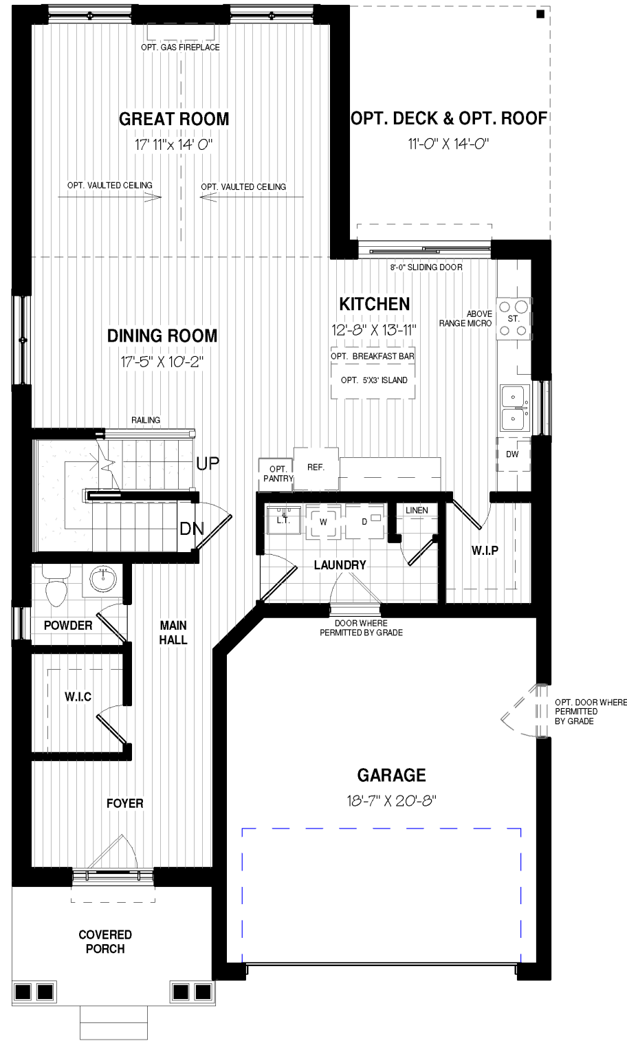
MAIN FLOOR PLAN-1201 sq.ft
