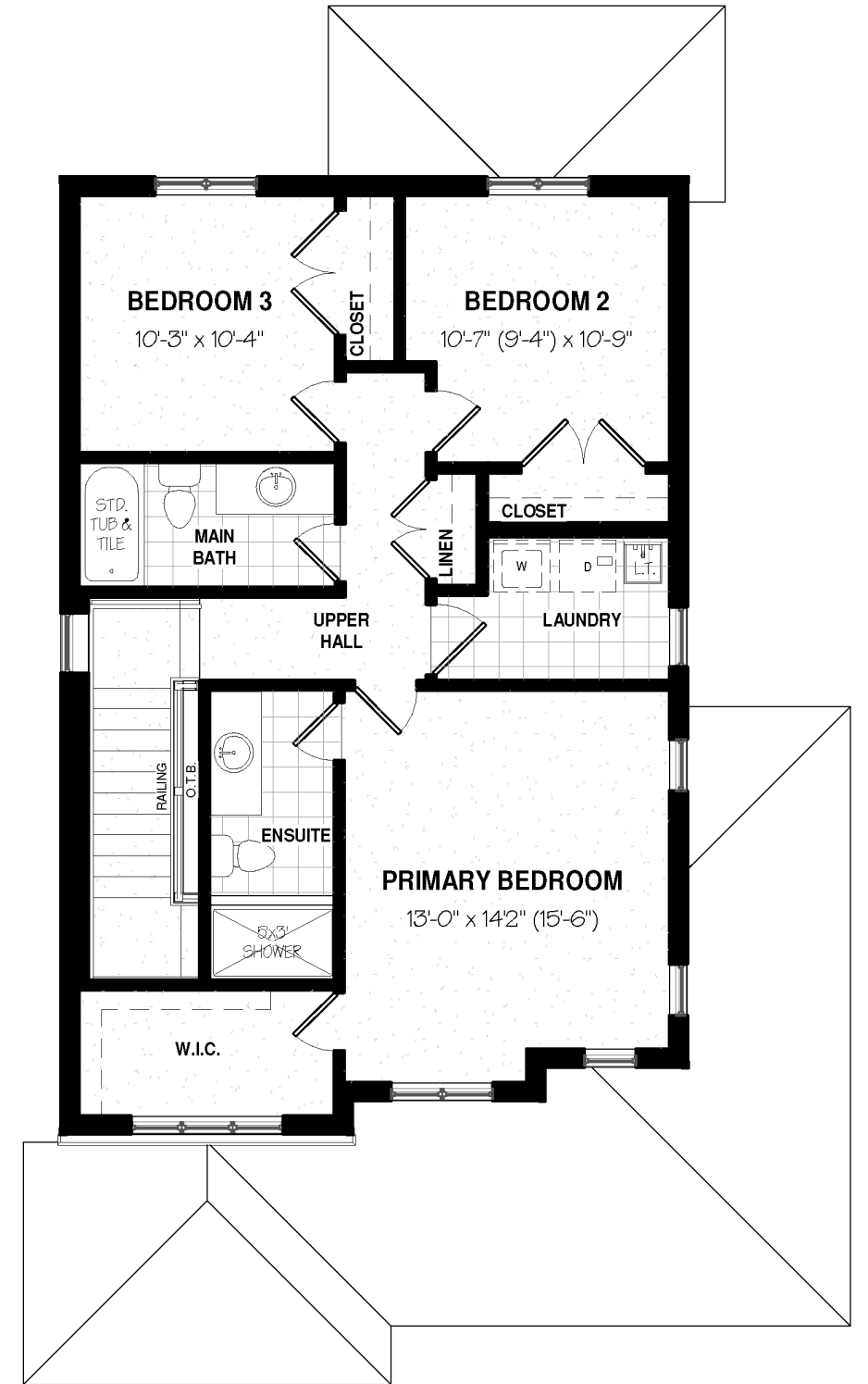
2ND FLOOR PLAN-864 sq. ft. OTB- 6 sq.ft.
