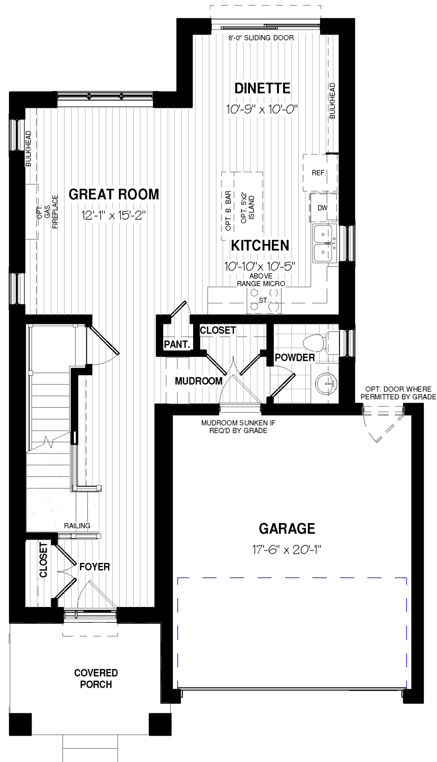
MAIN FLOOR PLAN-830 sq. ft.
