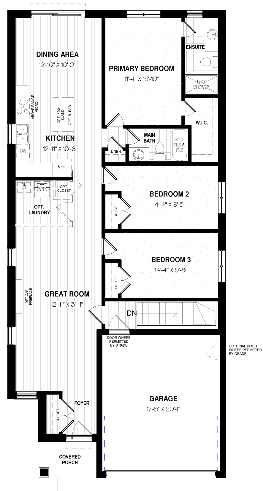
MAIN FLOOR PLAN-1635 sq. ft.
