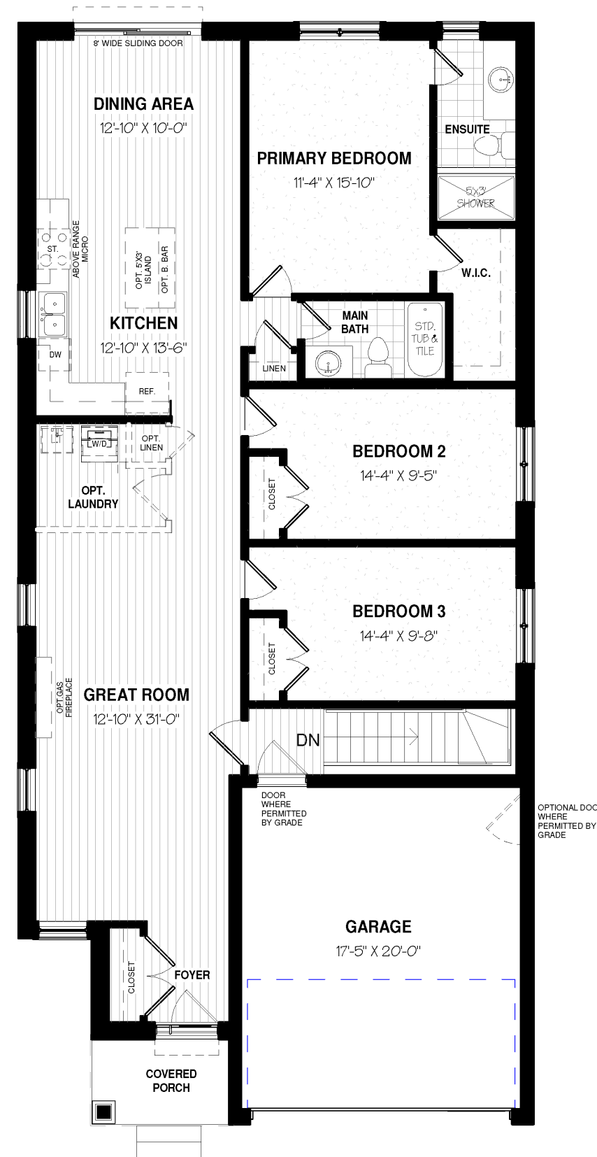
MAIN FLOOR PLAN-1635 sq. ft.
