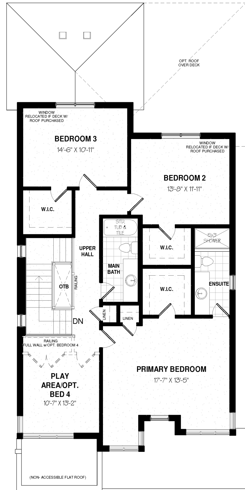
SECOND FLOOR PLAN-1243 sq.ft. OTB-14 sq.ft.
