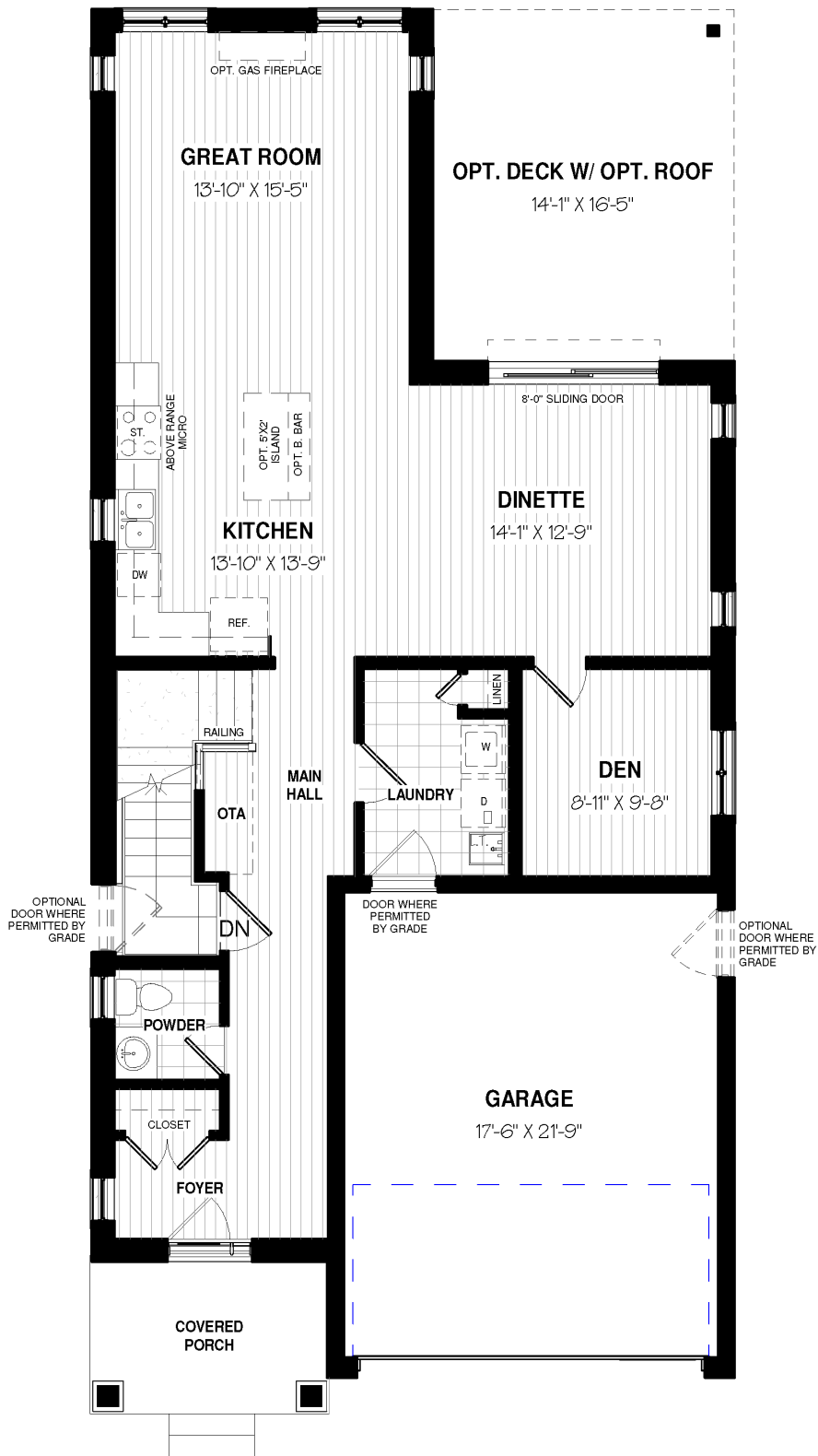
MAIN FLOOR PLAN-1208 sq.ft.
