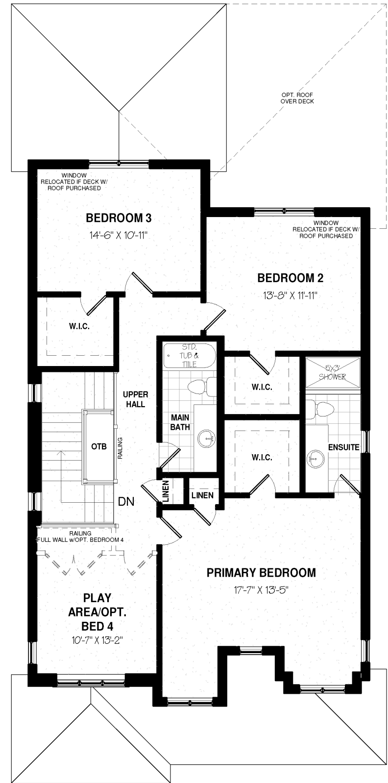
SECOND FLOOR PLAN-1243 sq.ft. OTB-14 sq.ft.
