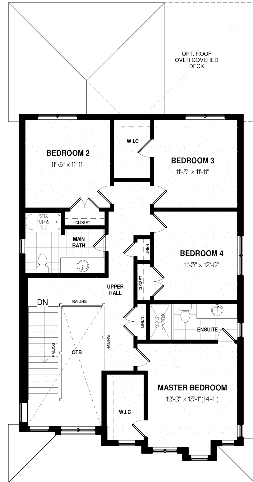
2ND FLOOR PLAN-1169 sq.ft. OTB-103 sq.ft.
