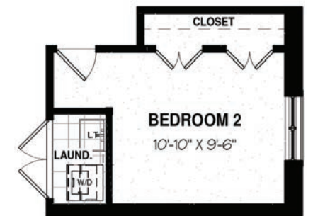
OPT. MAIN FLOOR LAUNDRY (BASEMENT LAUNDRY REMOVED IF PURCHASED)
