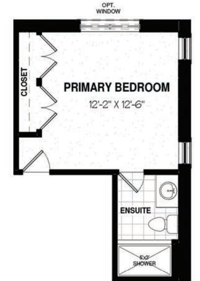
OPT. PRIMARY BEDROOM W/ ENSUITE LAYOUT
