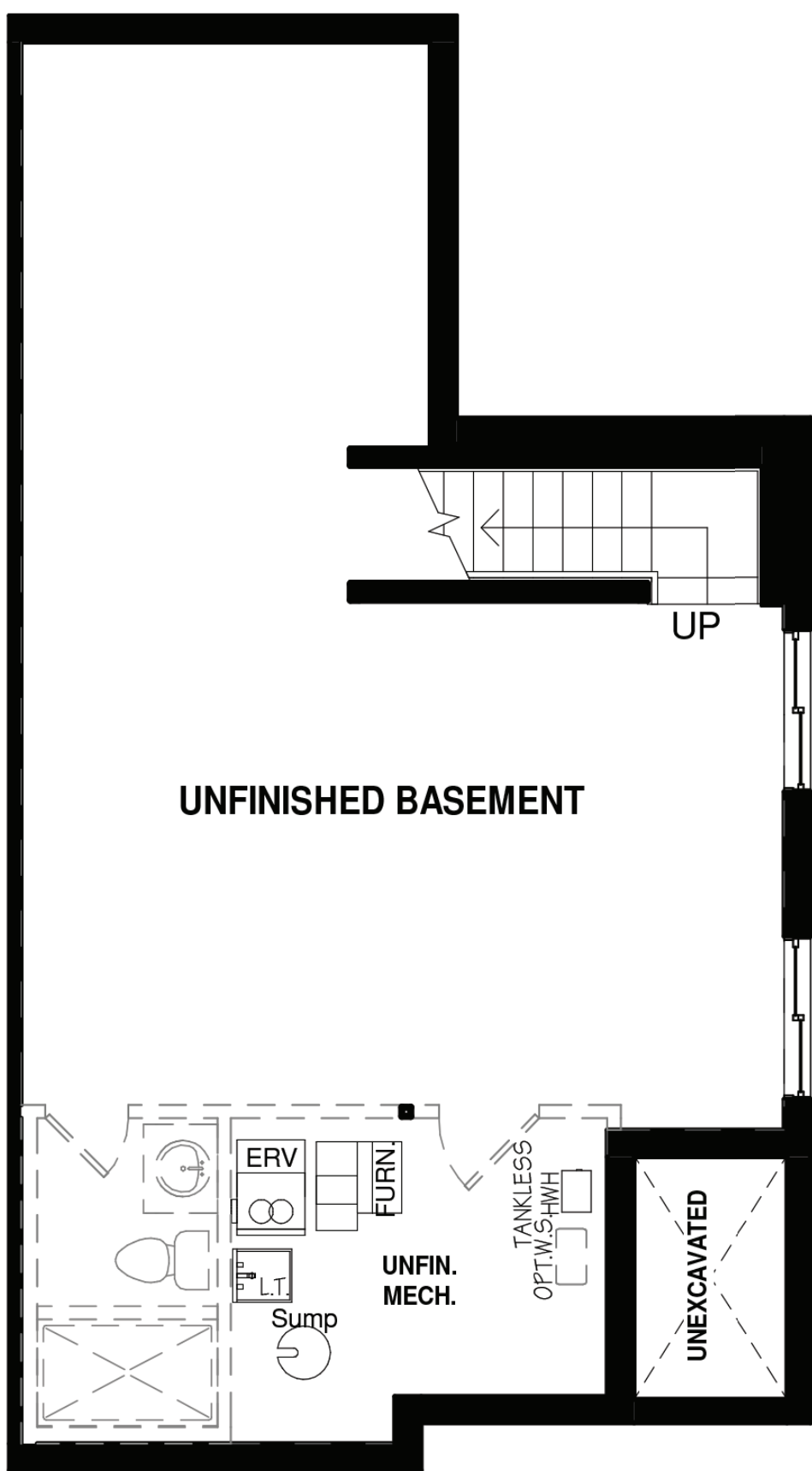
BASEMENT PLAN
