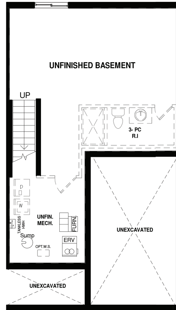
BASEMENT PLAN
