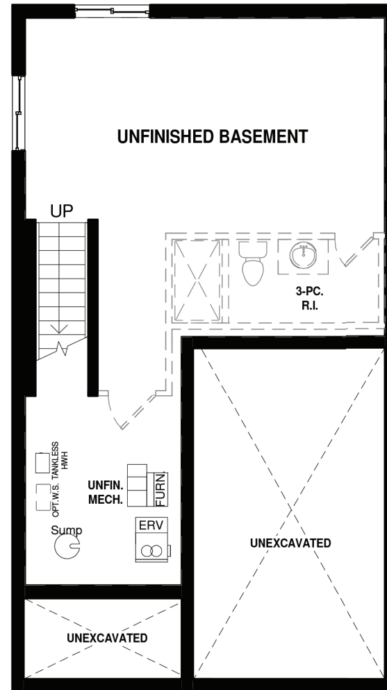
BASEMENT PLAN
