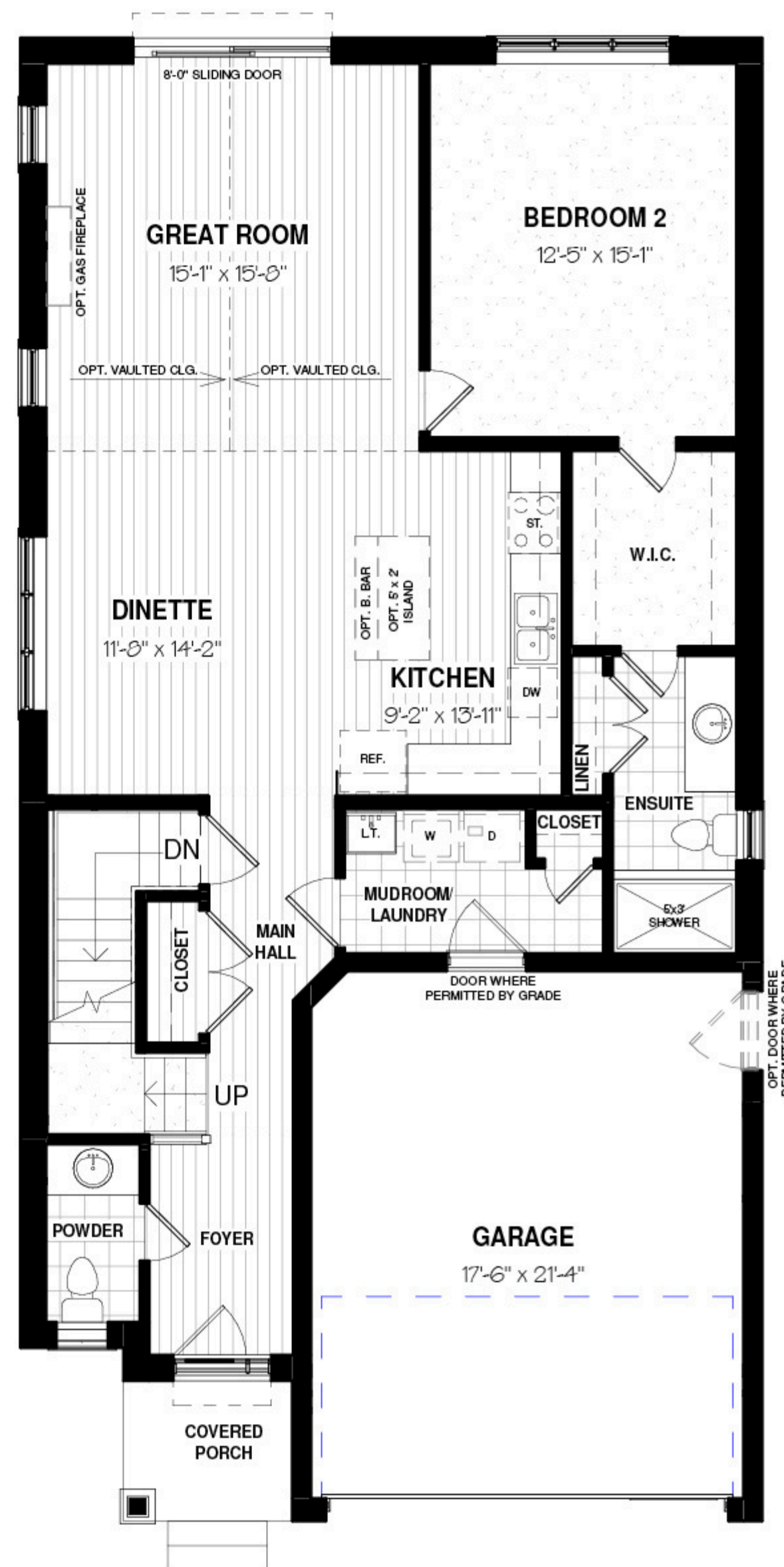
MAIN FLOOR PLAN - 1323 sq.ft.
