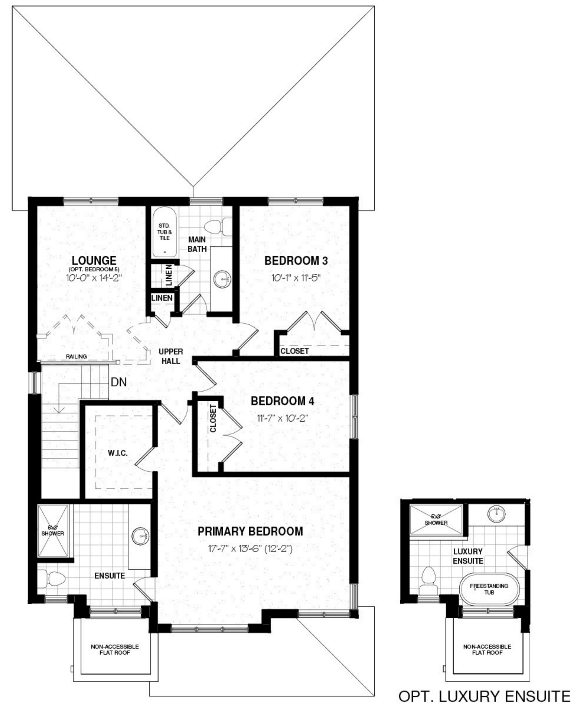
SECOND FLOOR PLAN - 1104 sq.ft.
