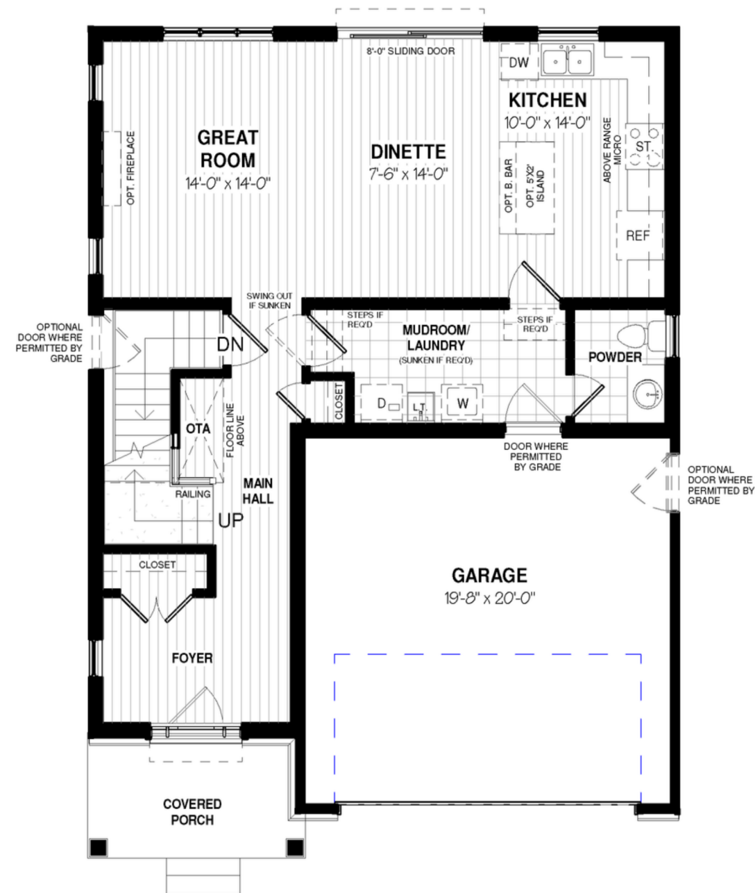
MAIN FLOOR - 905 SQ.FT.
