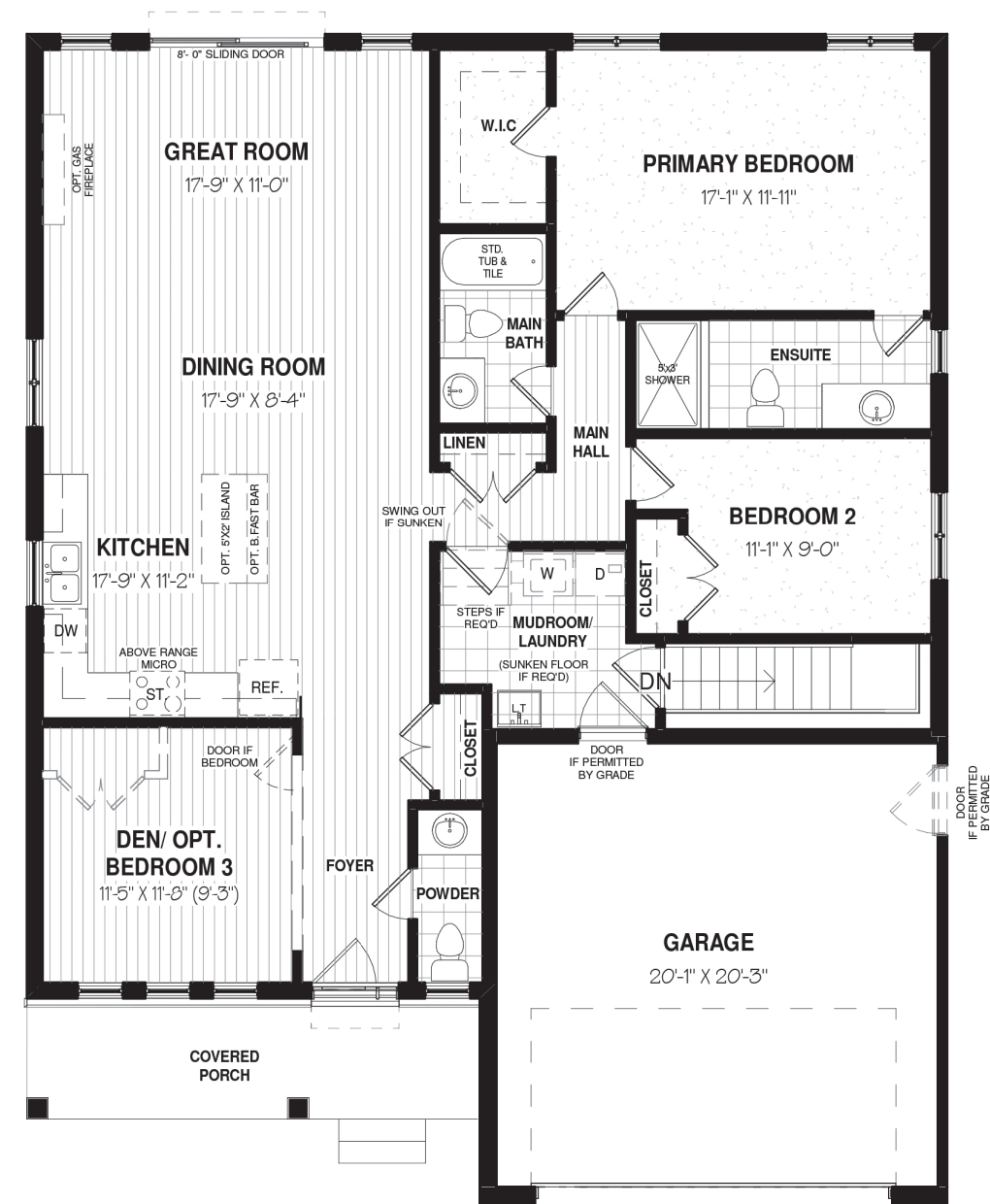
MAIN FLOOR - 1556 SQ.FT.
