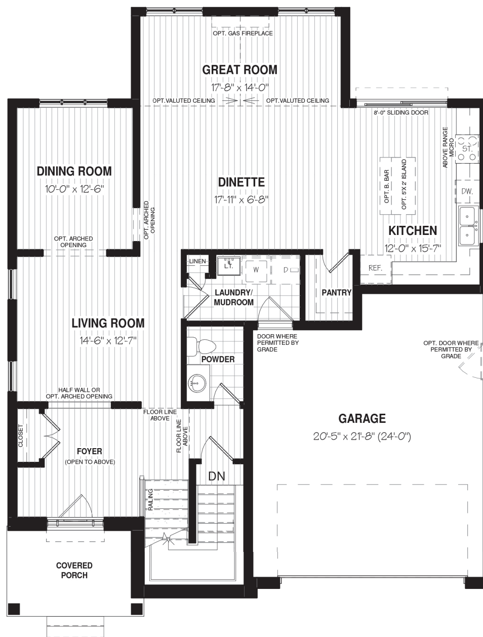
MAIN FLOOR - 1409 SQ.FT.
