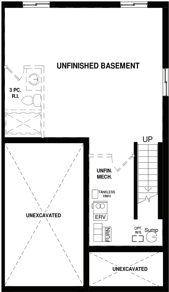
BASEMENT PLAN
