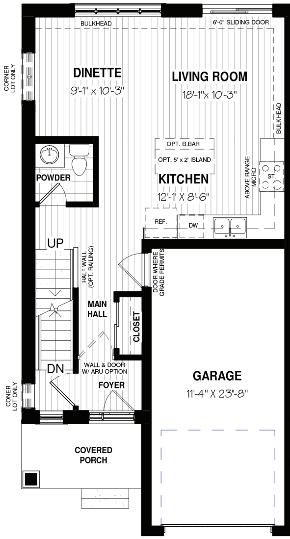
MAIN FLOOR 627 SQ FT
