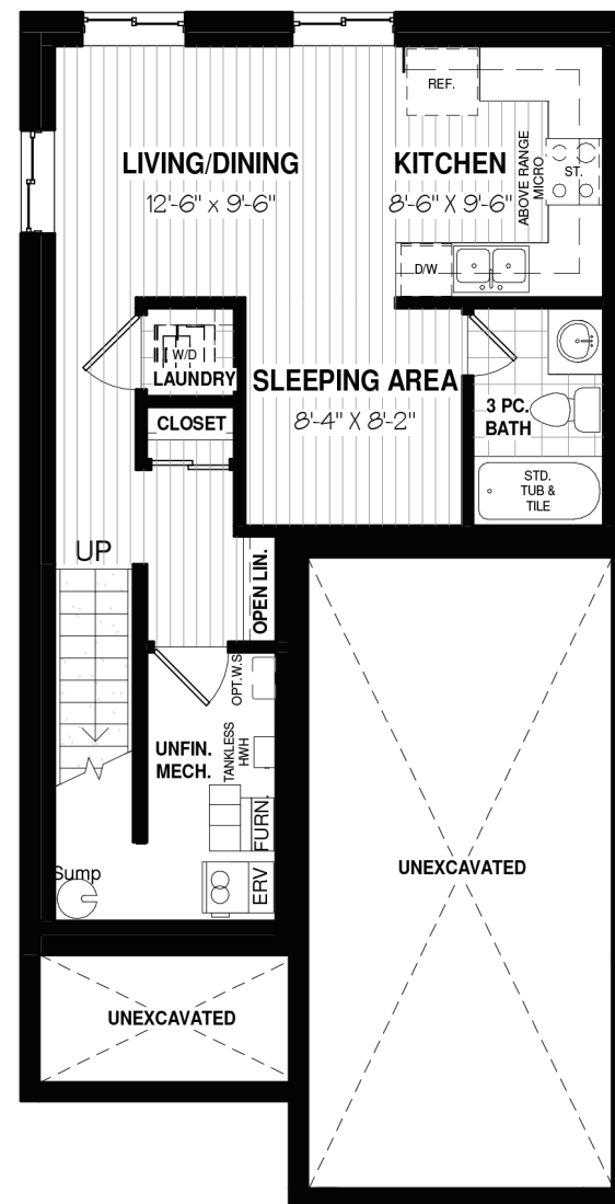
OPTIONAL BASEMENT APARTMENT PLAN 626 SQ FT
