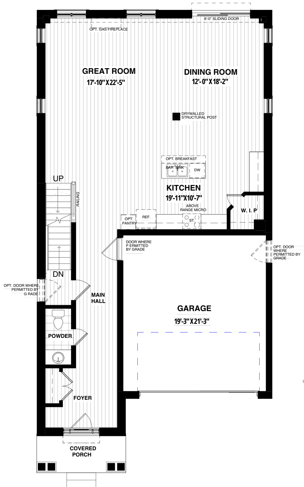
MAIN FLOOR PLAN - 1302 sq.ft.
